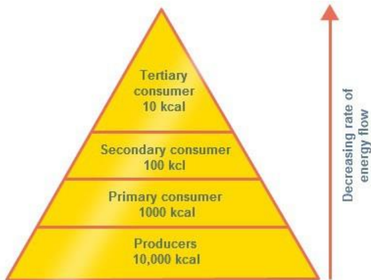
Figure 6: Upright pyramid of energy
